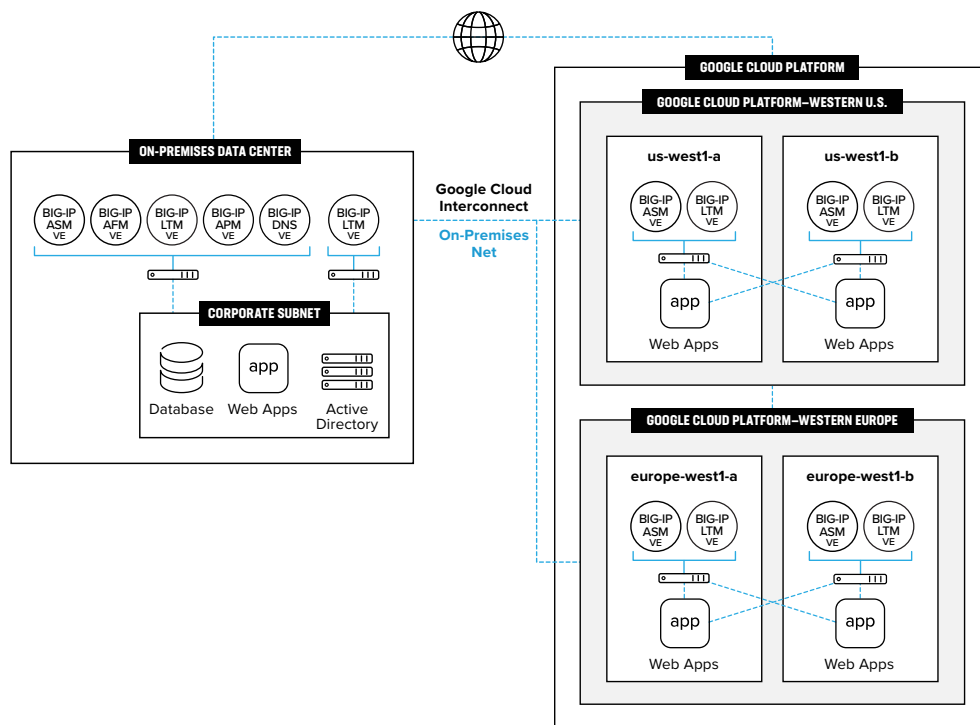
Figure 1: F5 offers consistent enterprise-class application services to applications located anywhere within hybrid-cloud architectures.
