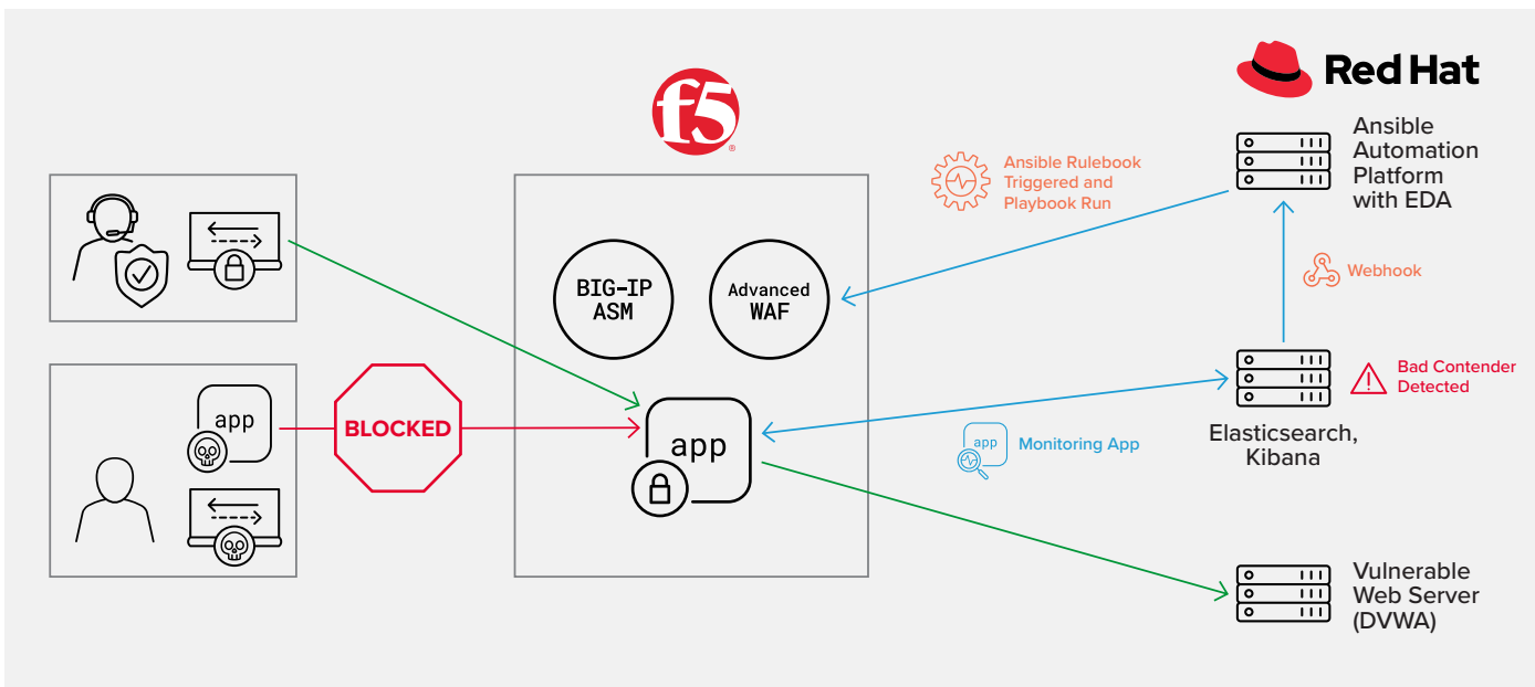
Figure 1: When suspicious activity is detected by Elasticsearch and Kibana, an Ansible Rulebook is triggered to take immediate action using BIG-IP Advanced WAF to block the malicious user.
