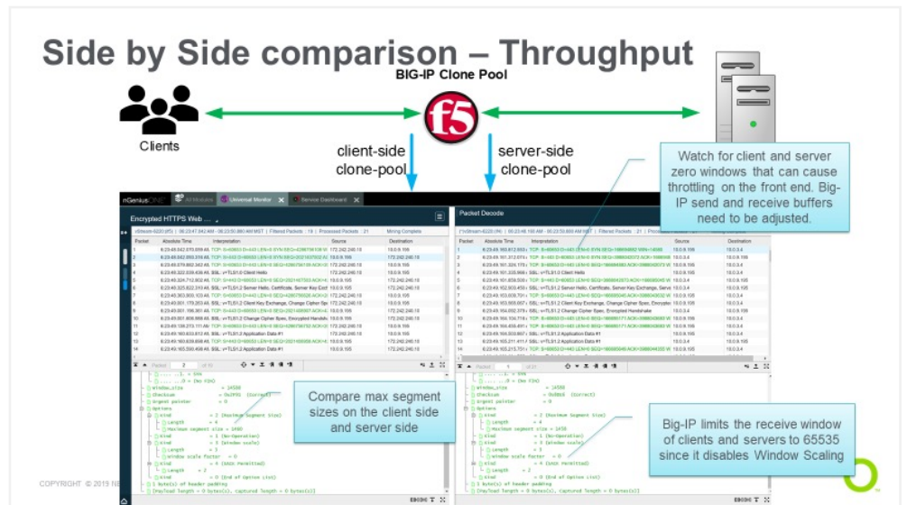
Figure 19: Session comparison from virtual server to pool throughput
