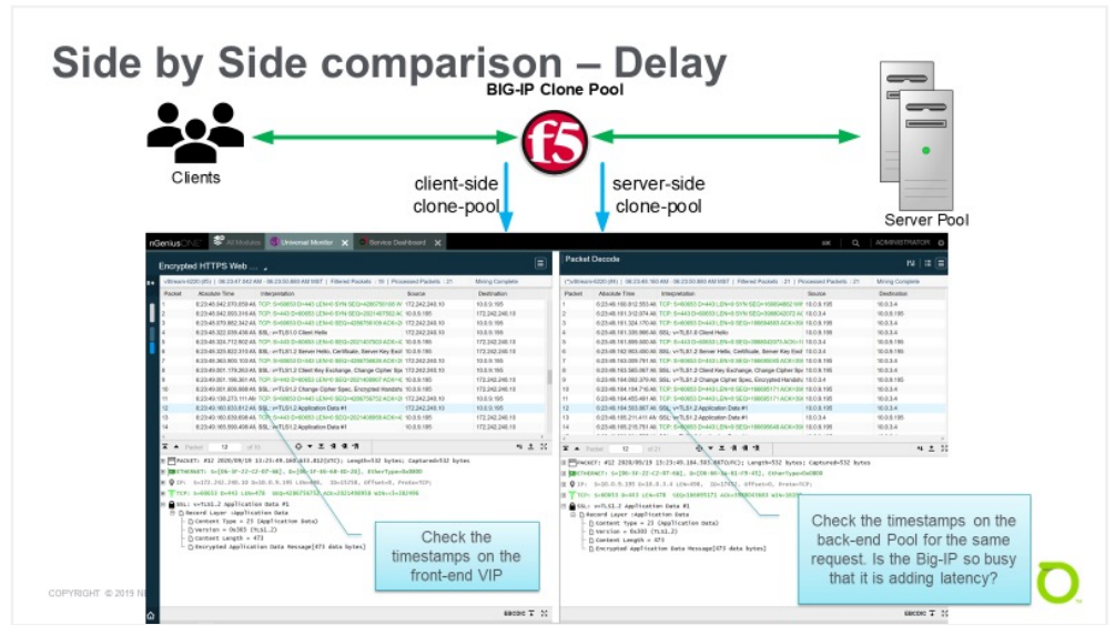
Figure 18: Session comparison from virtual server to pool delay
