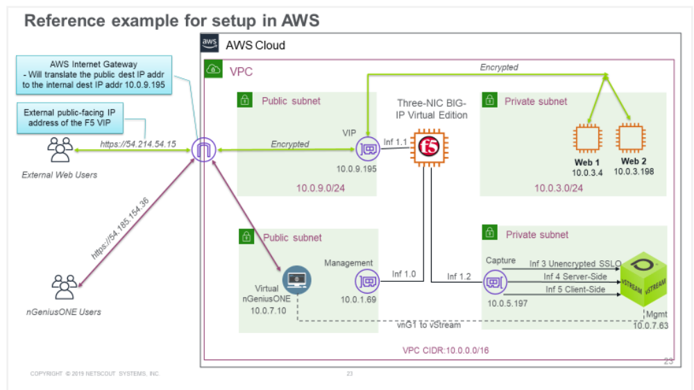
Figure 20: Reference example setup in AWS
